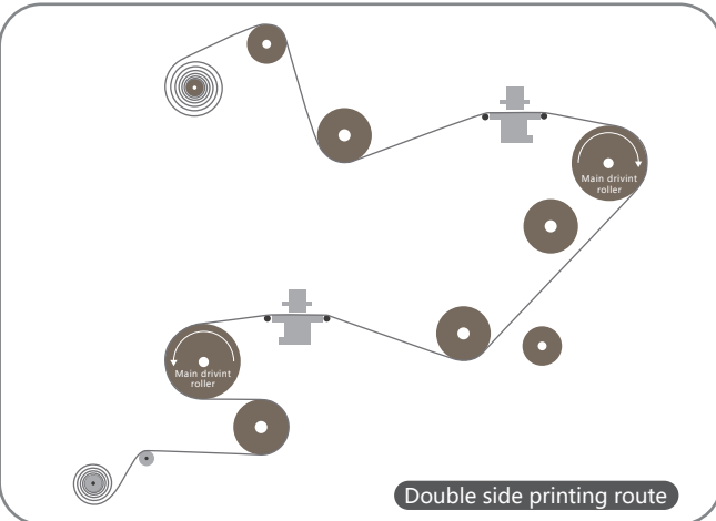
1 unit 8 rollers double sided structure
